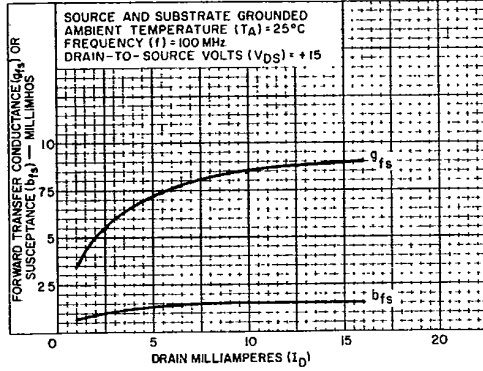
Fig. 7 - Forward Transadmittance ( y_{fs} ) vs Drain Current ( I_D )
